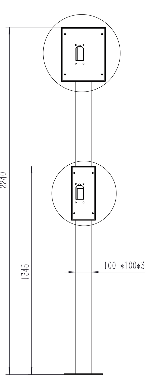
Front View
